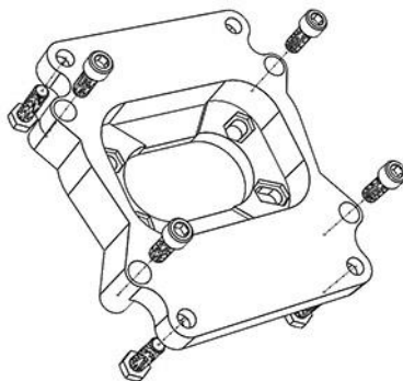
Quadrajet to 2300
