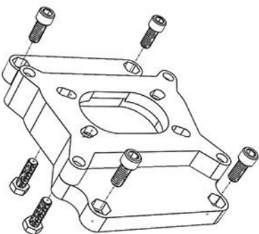
Carter to Quadrajet
