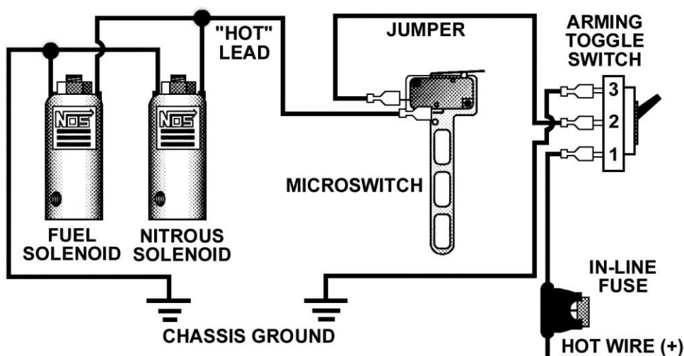
Figure 6 Wiring Schematic
