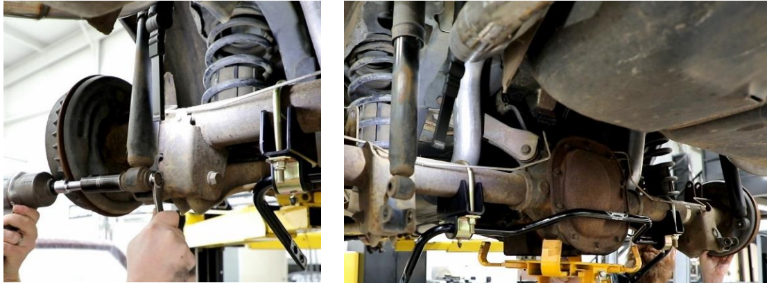
Figure 2 - Remove Lower Shock Bolts
