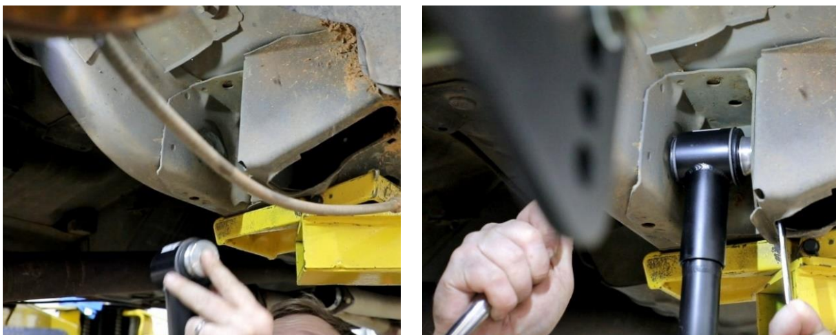
Figure 10 – Install Lower Swivel-Link™
