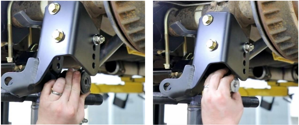
Figure 11 – Install Lower Swivel-Link™
