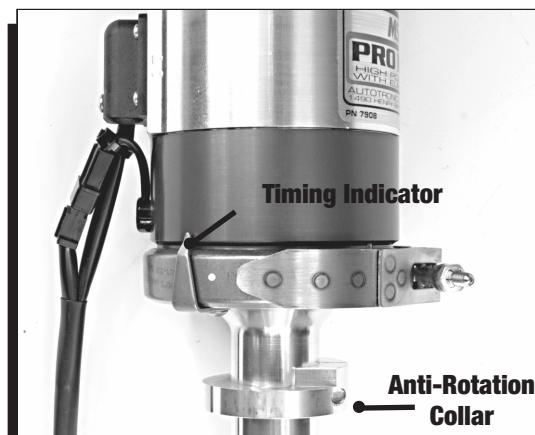
Figure 1 Positioning the Chevrolet Generator.
