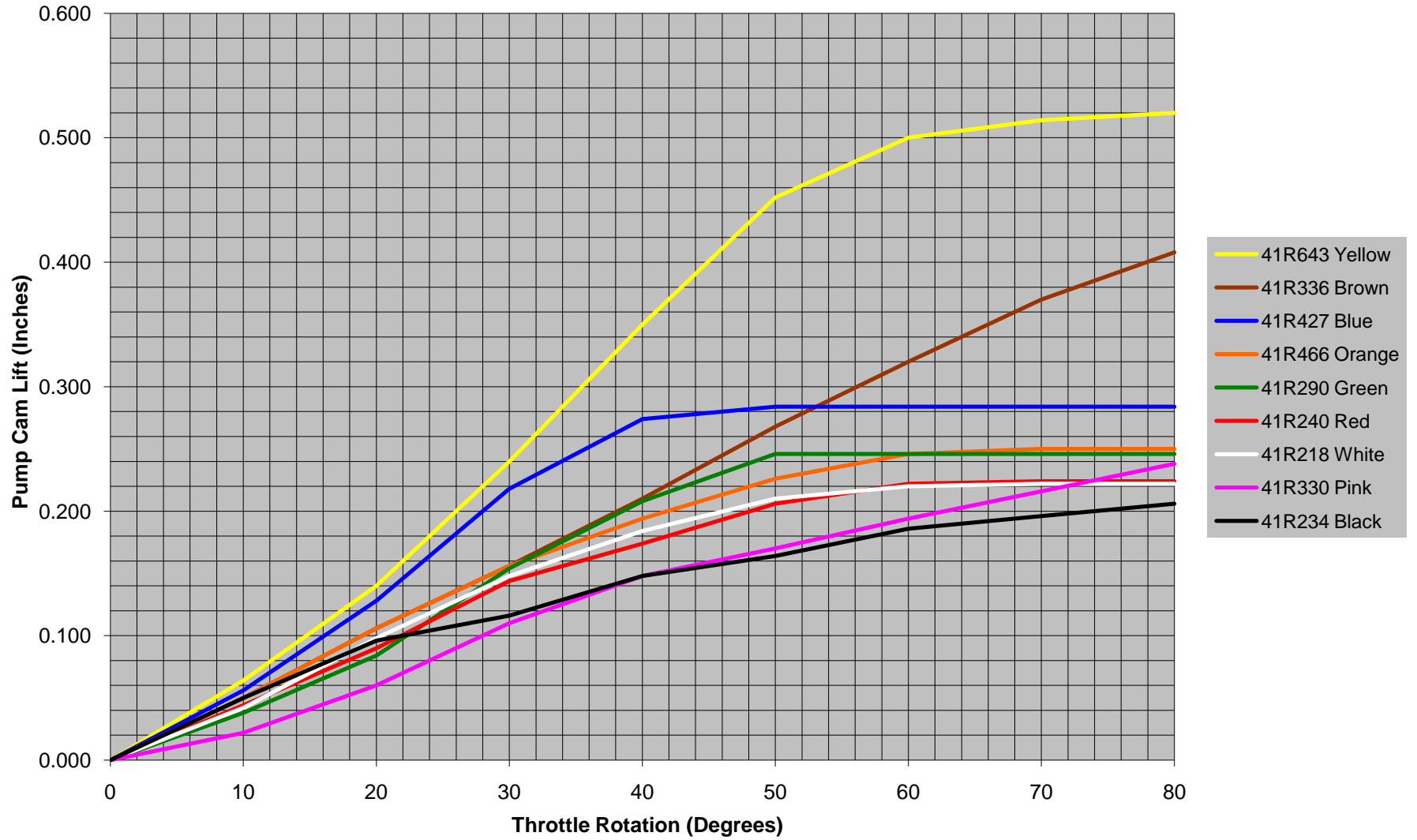
Pump Cam Lift vs. Throttle Position
