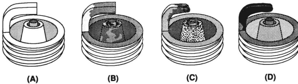
Figure 17 Spark Plug Condition
