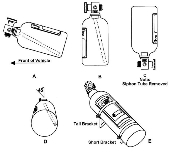
Figure 2 Nitrous Bottle Mounting Orientations
