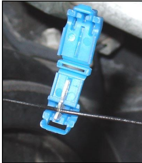
Figure 9 (T-Tap connector installation)
