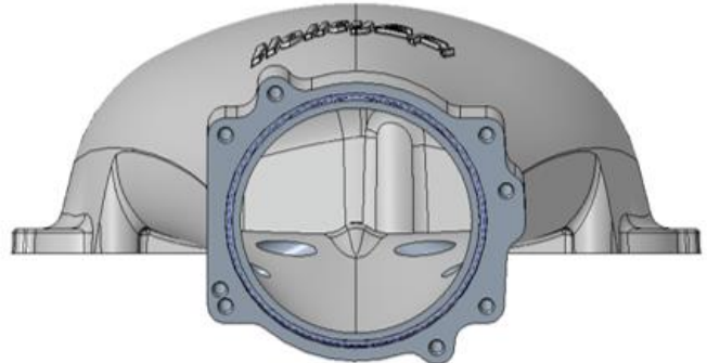
300-915 is designed to work with any of these Throttle types – throttle opening is 92mm in diameter:
