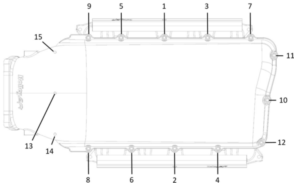
Plenum Top Torque Sequence for 300-910 and 300-915
