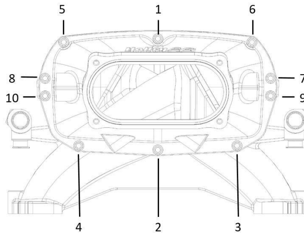
Throttle Body Flange Torque Sequence 300-911 & 300-912
