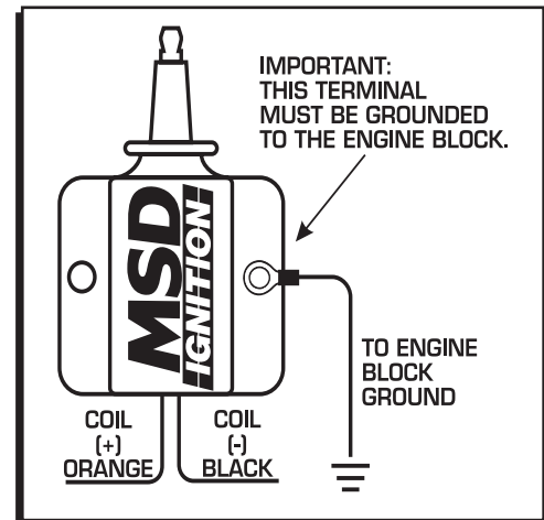
Figure 1 Grounding the Coil.
