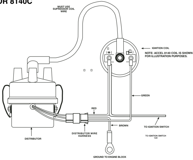
ACCEL POINTS ELIMINATOR WIRING DIAGRAM USING 12V IGNITION FEED AND AN ACCEL 140108, 8140 OR 8140C
