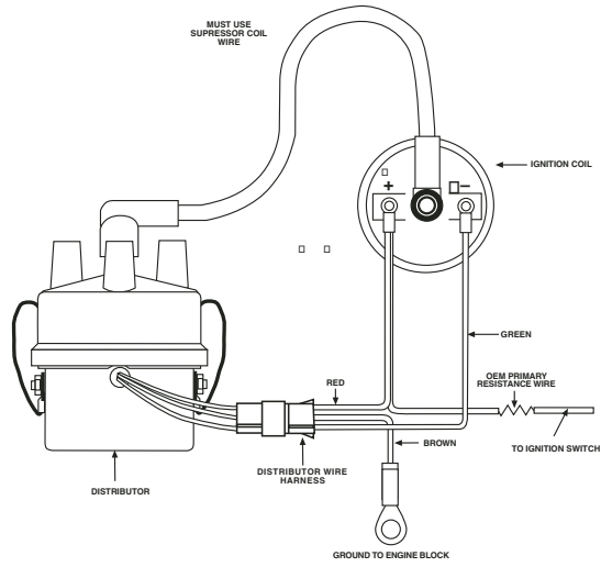
ACCEL POINTS ELIMINATOR WIRING DIAGRAM USING OEM PRIMARY RESISTANCE WIRE
