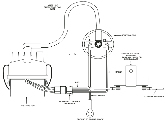
ACCEL POINTS ELIMINATOR WIRING DIAGRAM USING BALLAST RESISTOR
