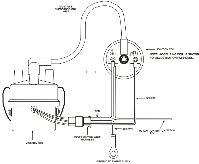
ACCEL POINTS ELIMINATOR A 12V IGNITION FEED AND AN ACCEL P/N 140305, 8140 OR 8140C SUPERSTOCK CANISTER COIL.
