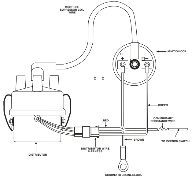
ACCEL POINTS ELIMINATOR WIRING DIAGRAM USING OEM PRIMARY RESISTANCE WIRE
