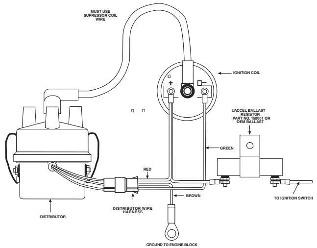
ACCEL POINTS ELIMINATOR WIRING DIAGRAM USING A BALLAST RESISTOR
