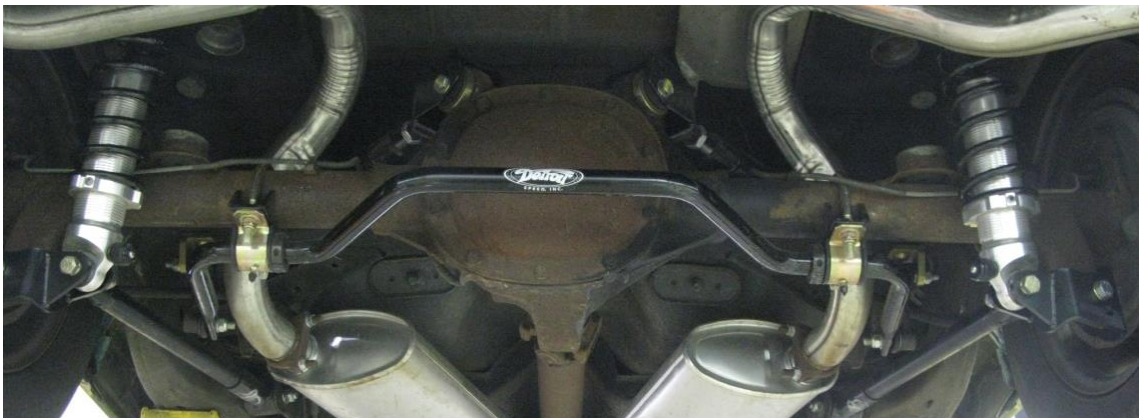
Figure 3 - Completed Coilover Installation
