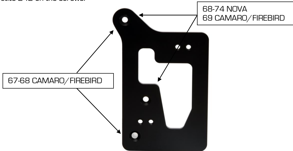
Figure 1 - C6 Throttle Pedal Bracket
