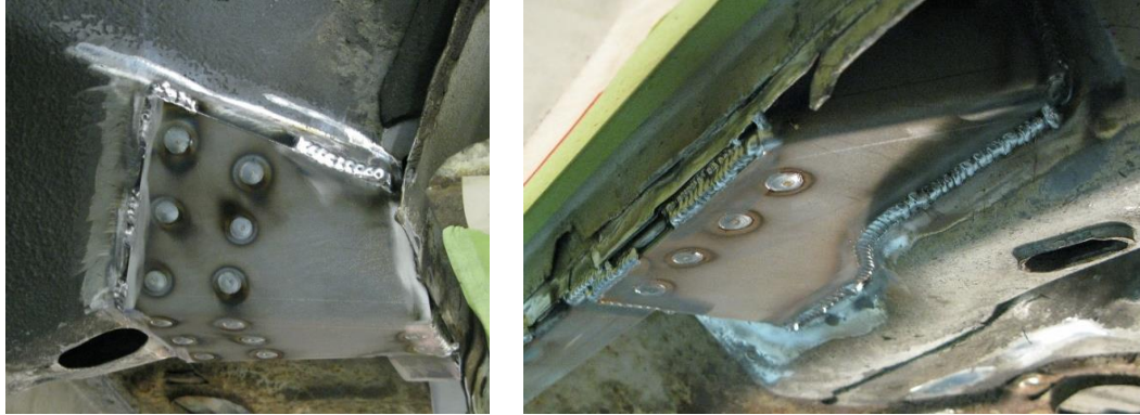
Figure 29 – Weld Doubler Plates
