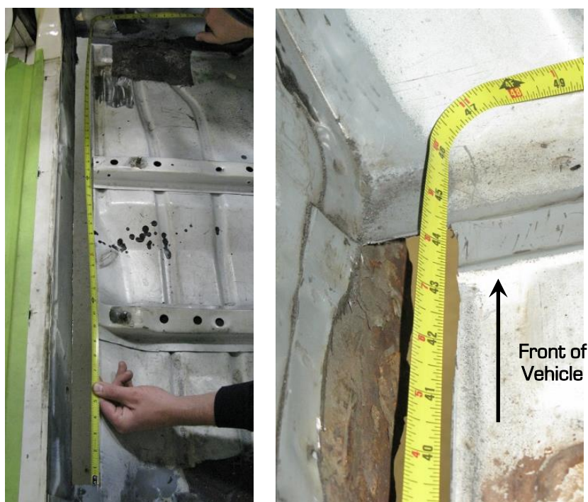
Figure 19 - Cut Driver Side Floor Pan
