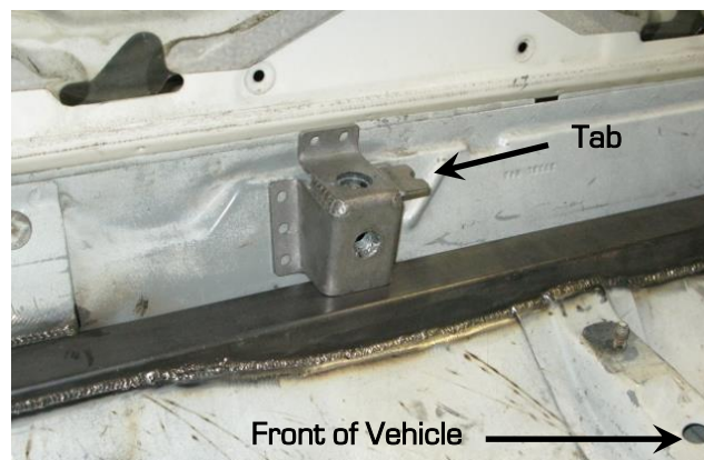
Figure 31 – Seat Belt Mount
