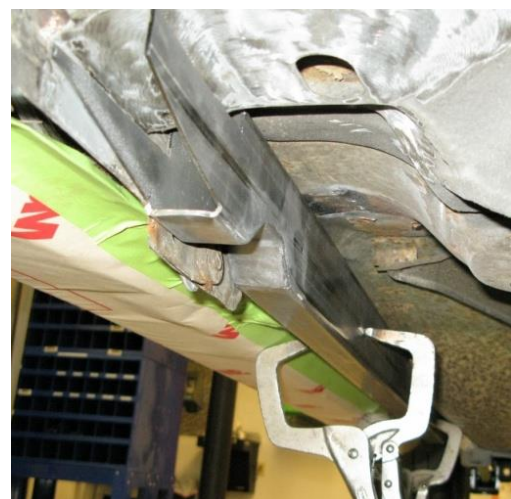
Figure 10 - Clamp Connector
