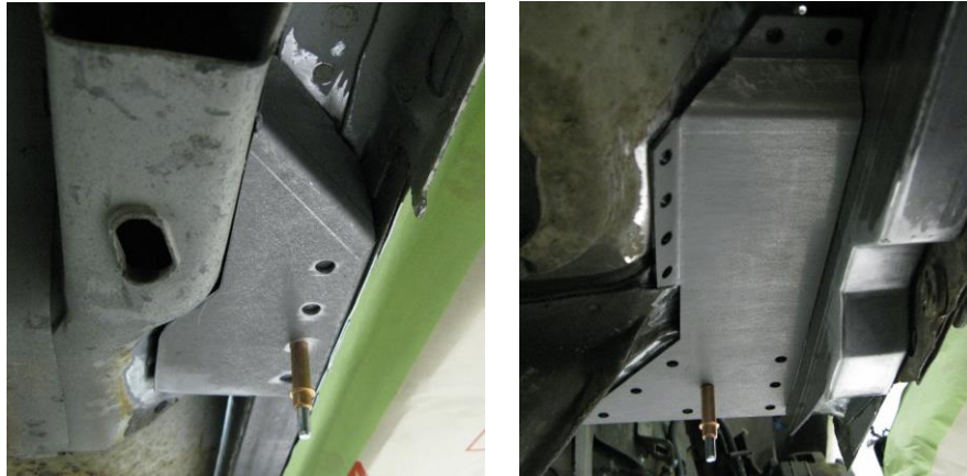
Figure 11 - Rear & Front Doubler Plate
