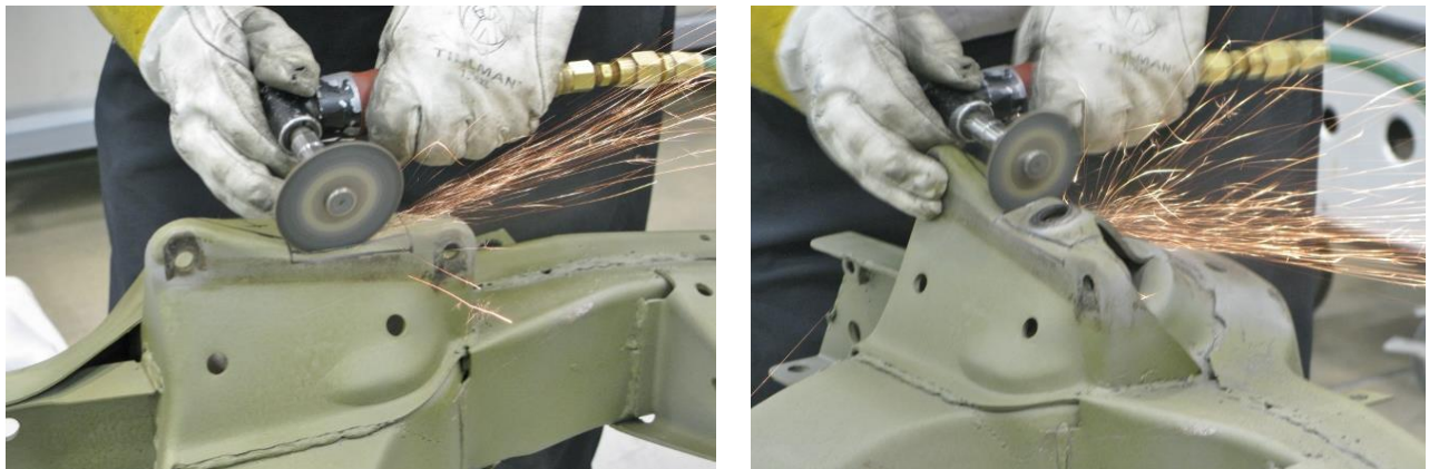
Figure 5 - Cut Factory Upper Shock Mount
